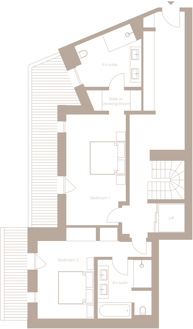
Grand residence ground floor
